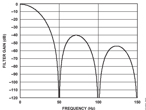
Figure 59. Sinc3 Filter Response
