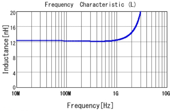
■ LQP15MN12NG02 L
