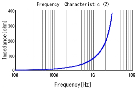
■ LQP15MN12NG02 |Z|
