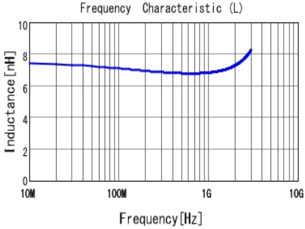
■ LQP03TN6N8H02 L
