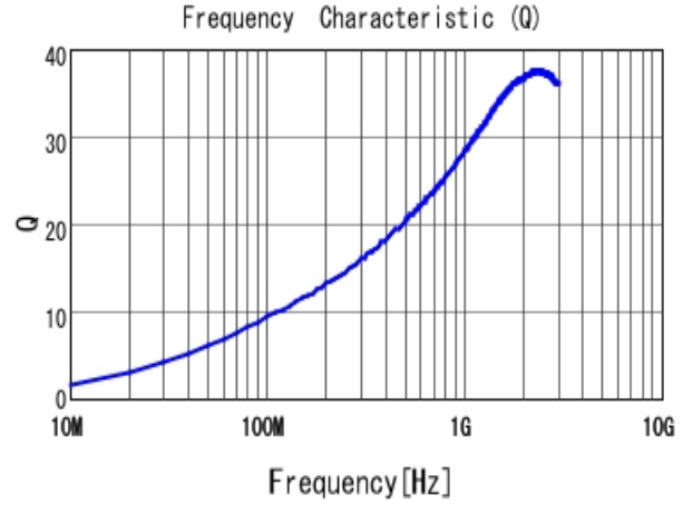
■ LQP03TN6N8H02 Q
