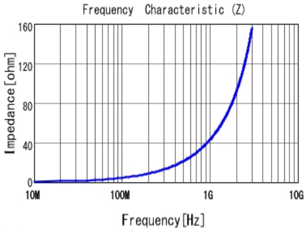
■ LQP03TN6N8H02 |Z|
