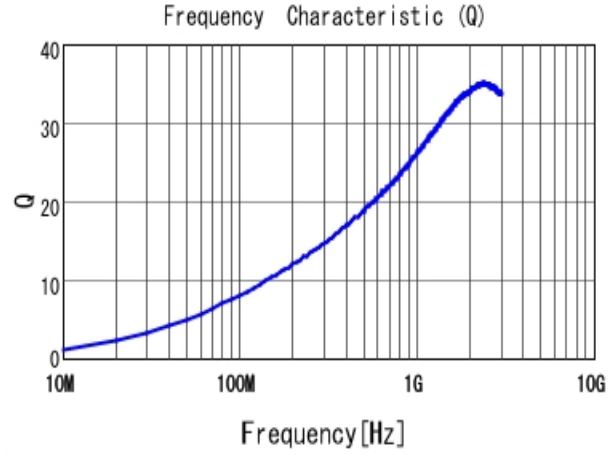
■ LQP03TN6N2J02 Q
