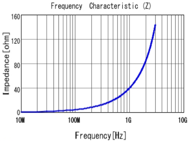
■ LQP03TN6N2J02 |Z|
