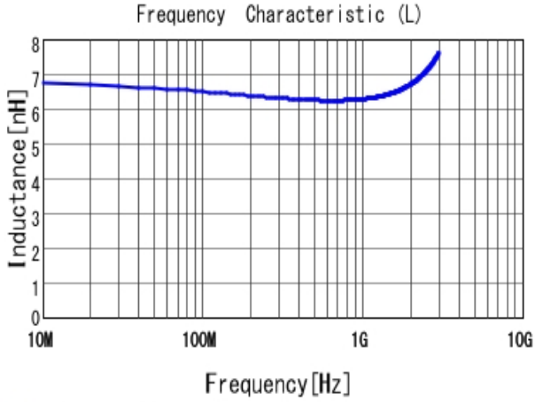
■ LQP03TN6N2J02 L
