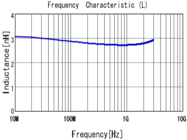
■ LQP03TN2N7B02 L
