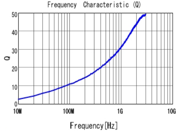
■ LQP03TN2N7B02 Q
