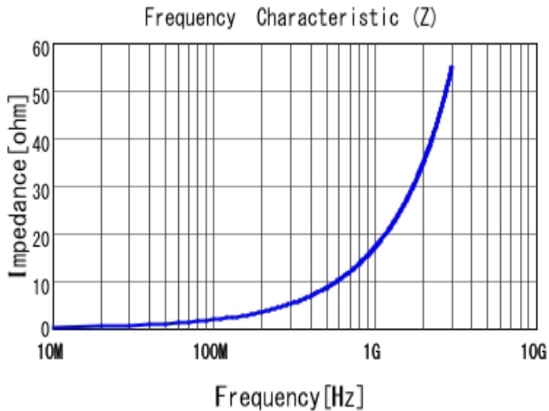
■ LQP03TN2N7B02 |Z|
