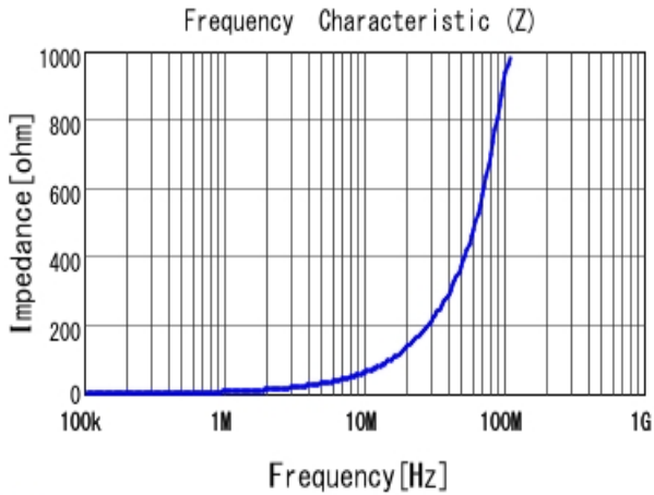
■ LQM21PN1R0MC0 |Z|
