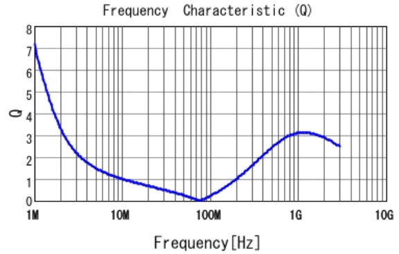
■ LQM21DN100N00 Q
