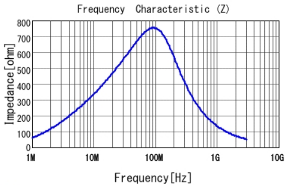
■ LQM21DN100N00 |Z|
