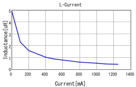
■ LQM18PN4R7MFR L-Current 20degC
