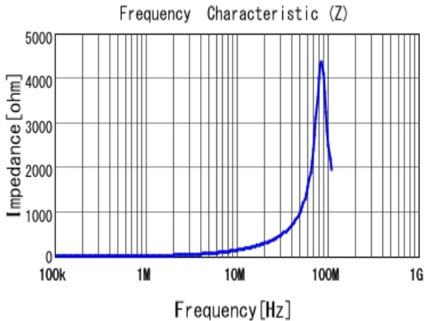
■ LQH43PN2R2M26 |Z|
