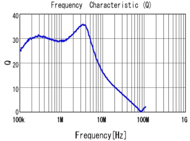
■ LQH43PN2R2M26 Q
