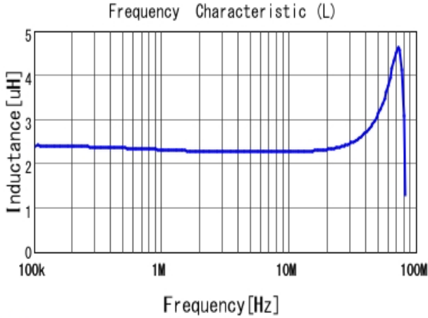
■ LQH43PN2R2M26 L
