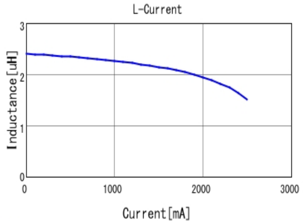
■ LQH43PN2R2M26 L-Current 20degC
