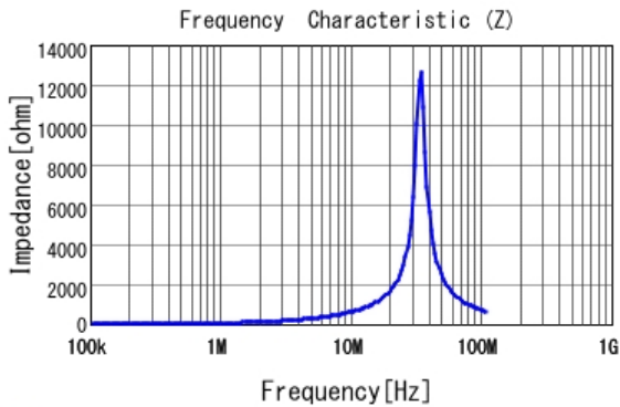
■ LQH43PN100M26 |Z|
