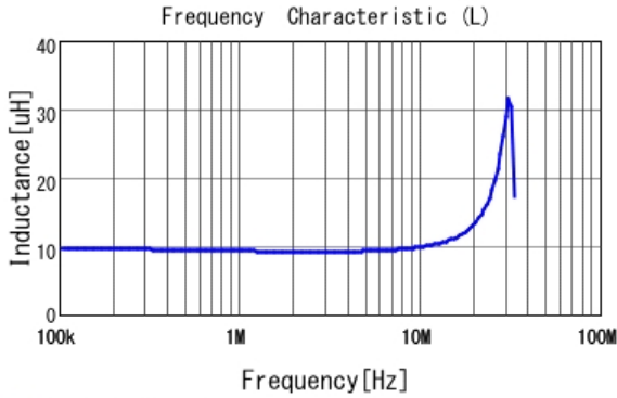
■ LQH43PN100M26 L
