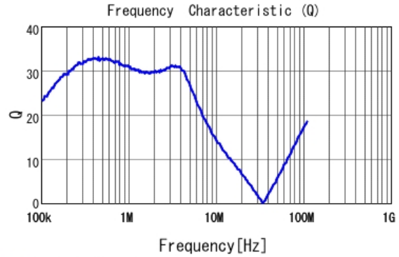
■ LQH43PN100M26 Q
