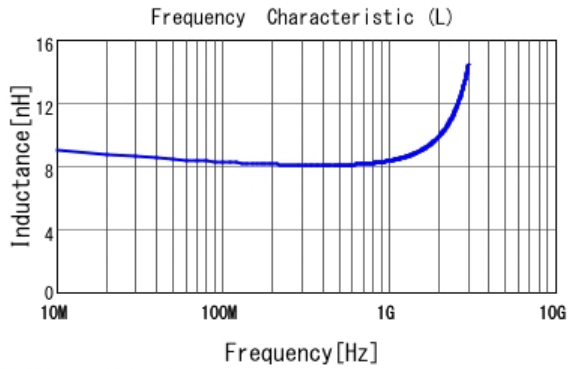
■ LQG18HN8N2J00 L
