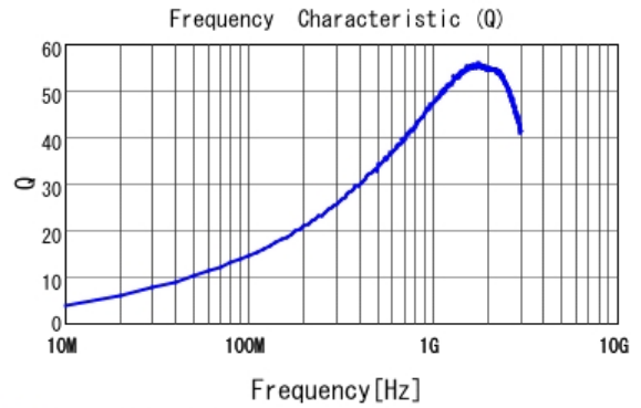
■ LQG18HN8N2J00 Q
