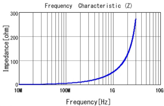
■ LQG18HN8N2J00 |Z|
