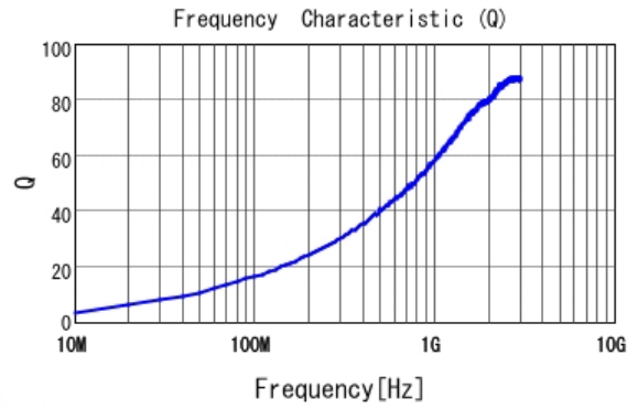
■ LQG18HN3N3S00 Q
