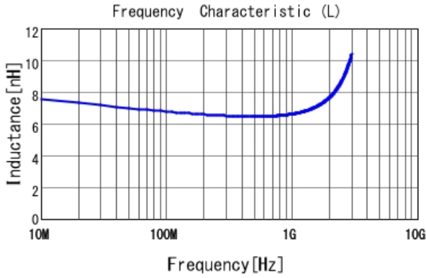
■ LQG15HS6N8J02 L
