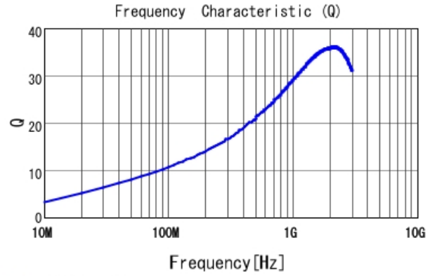
■ LQG15HS6N8J02 Q
