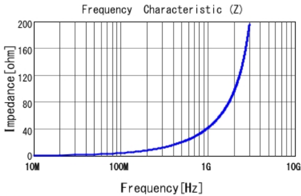
■ LQG15HS6N8J02 |Z|
