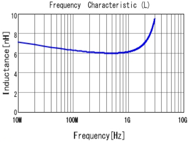
■ LQG15HS6N2S02 L
