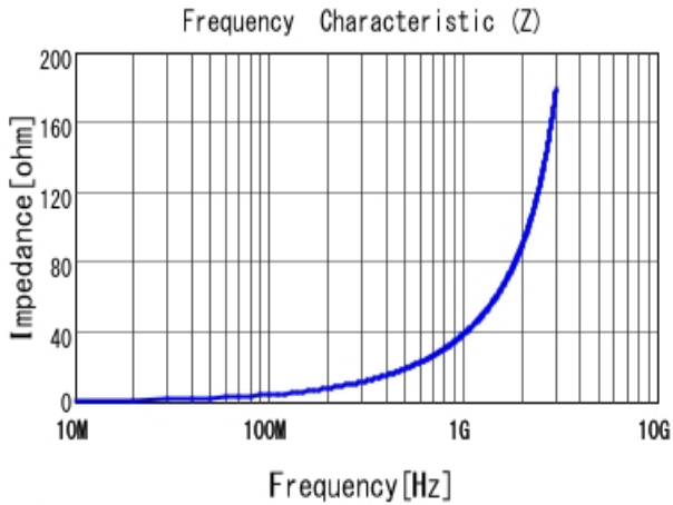
■ LQG15HS6N2S02 |Z|
