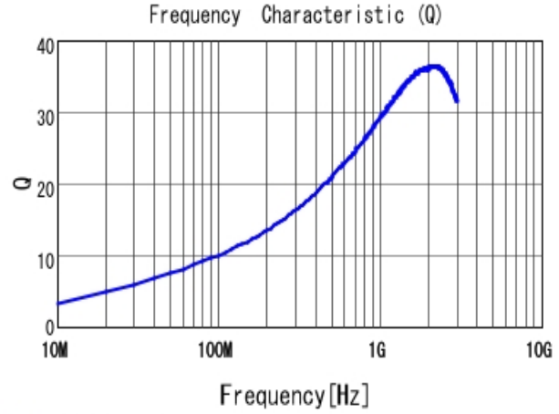
■ LQG15HS6N2S02 Q
