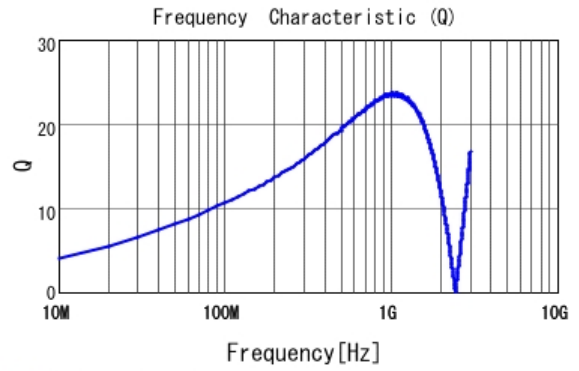
■ LQG15HS22NJ02 Q
