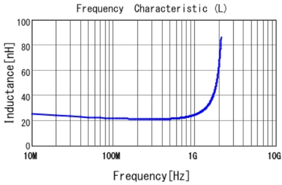
■ LQG15HS22NJ02 L
