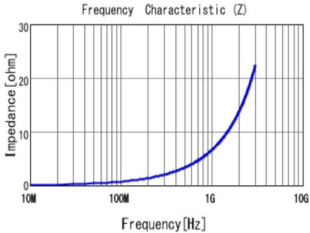
■ LQG15HS1N1S02 |Z|
