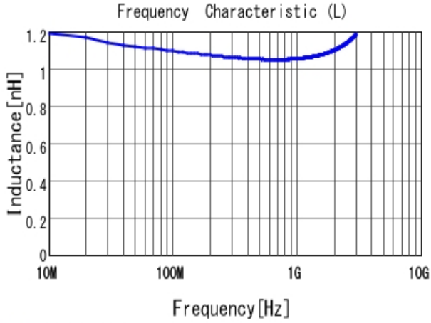
■ LQG15HS1N1S02 L
