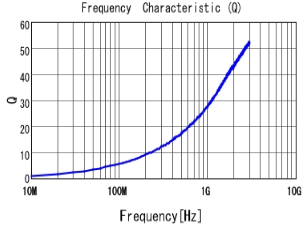
■ LQG15HS1N1S02 Q
