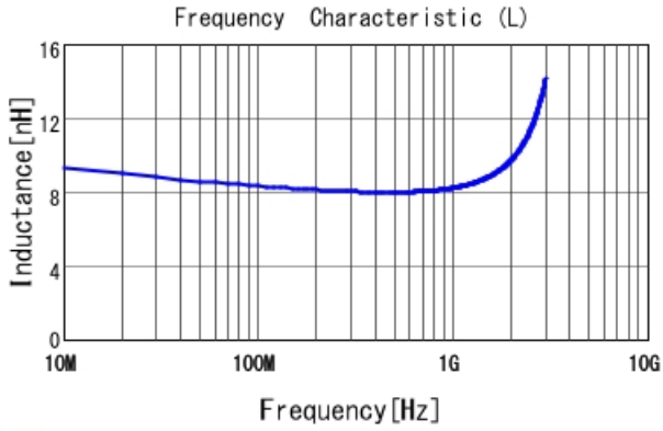
■ LQG15HN8N2J02 L
