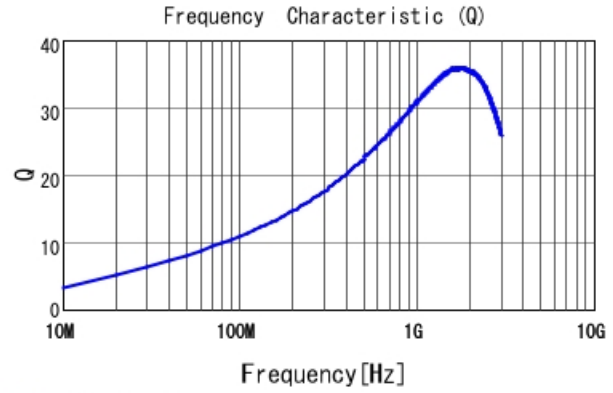
■ LQG15HN8N2J02 Q
