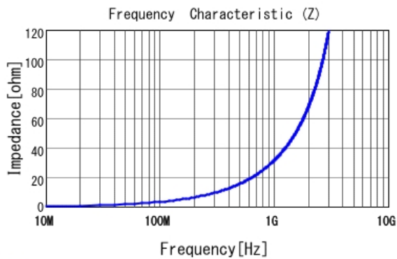
■ LQG15HN5N1S02 |Z|
