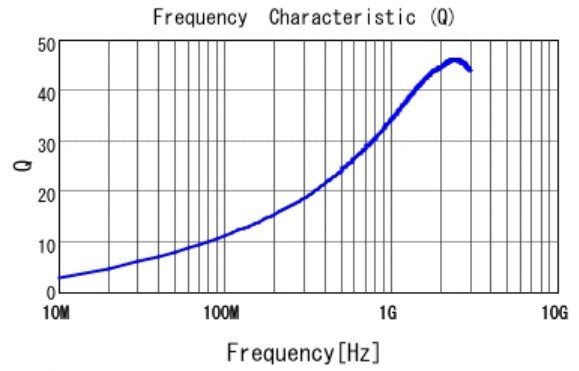
■ LQG15HN5N1S02 Q
