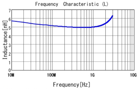
■ LQG15HN5N1S02 L
