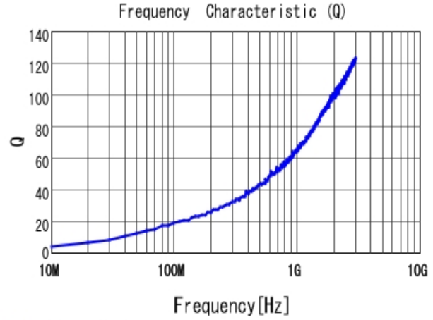
■ LQG15HN1N0S02 Q
