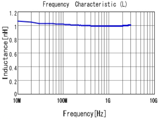
■ LQG15HN1N0S02 L
