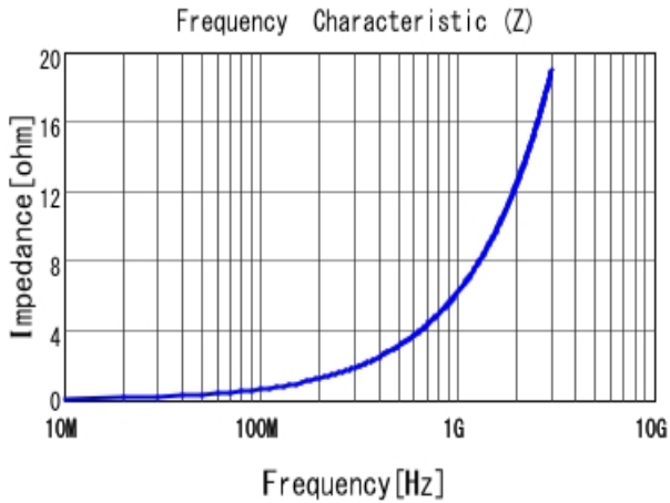
■ LQG15HN1N0S02 |Z|
