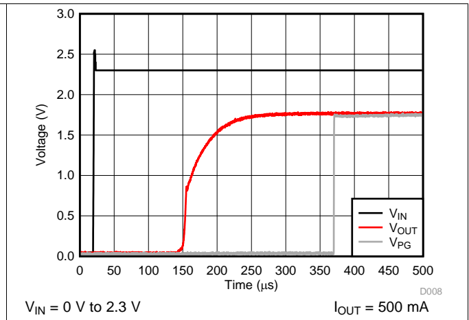
Figure 8. LP5912-1.8 Power Up
