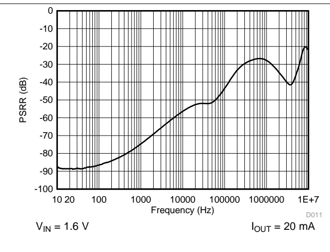
Figure 20. LP5912-0.9 PSRR vs Frequency
