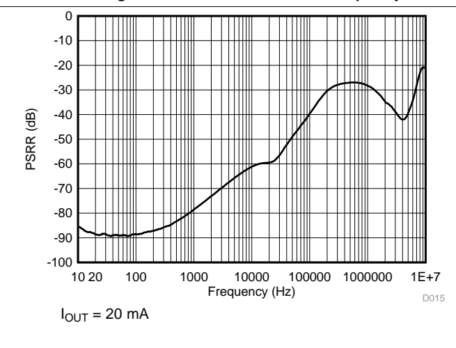
Figure 24. LP5912-3.3 PSRR vs Frequency
