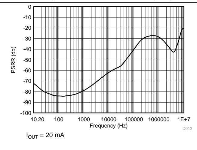
Figure 22. LP5912-1.8 PSRR vs Frequency
