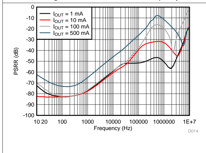
Figure 23. LP5912-1.8 PSRR vs Frequency
