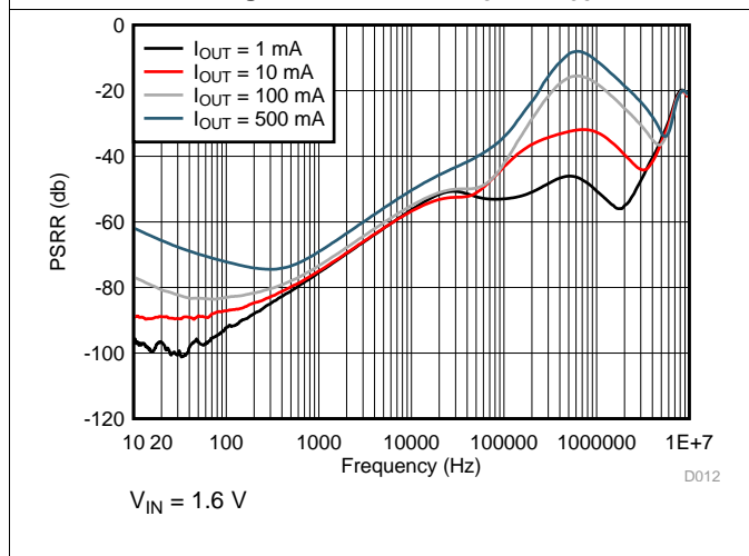
Figure 21. LP5912-0.9 PSRR vs Frequency
