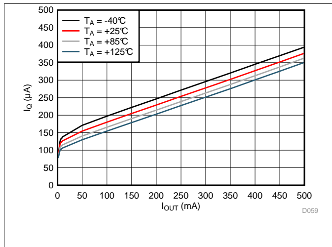
Figure 19. LP5912-3.3 I_{qND} vs I_{OUT}
