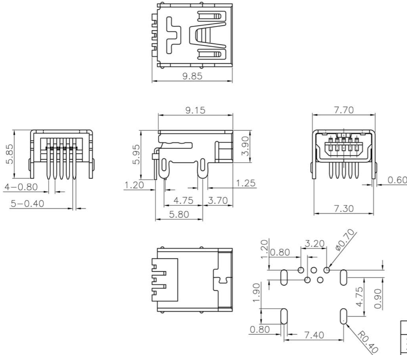
PCB LAYOUT
