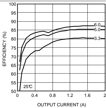
Figure 9. Efficiency 42-V Input
