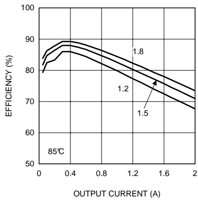
Figure 15. Efficiency 5-V Input at 85°C
