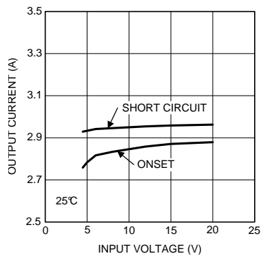
Figure 29. Current Limit 1.8 V OUT at 25°C
