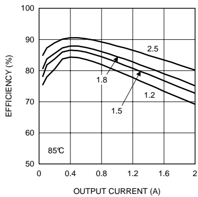
Figure 17. Efficiency 6-V Input at 85°C
