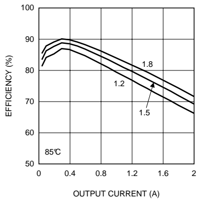
Figure 13. Efficiency 4.5-V Input at 85°C
