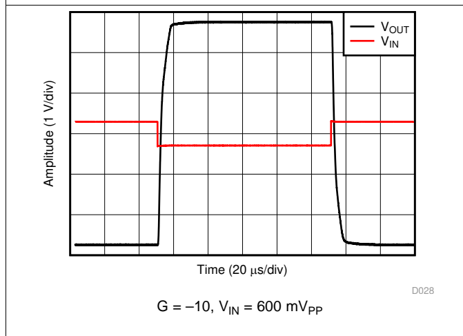
Figure 23. Overload Recovery
