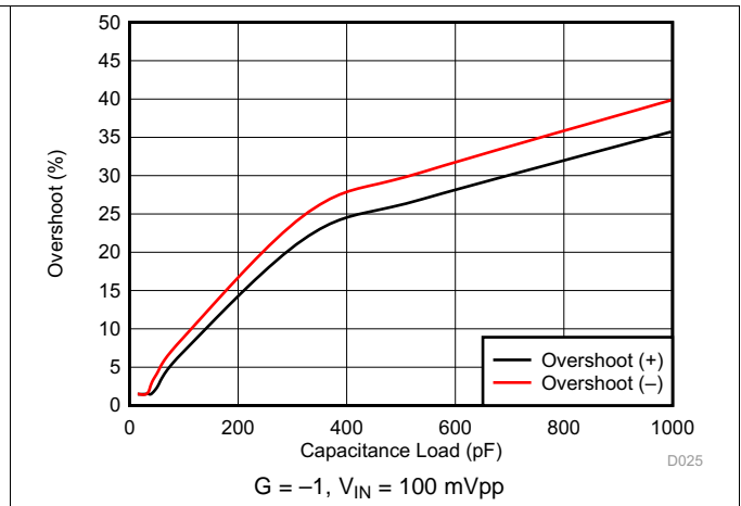
Figure 20. Small Signal Overshoot vs Capacitive Load
