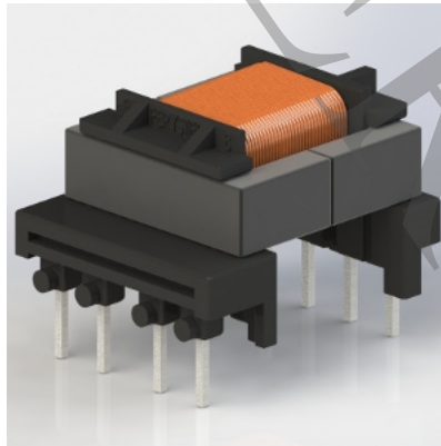
Transformer's model
