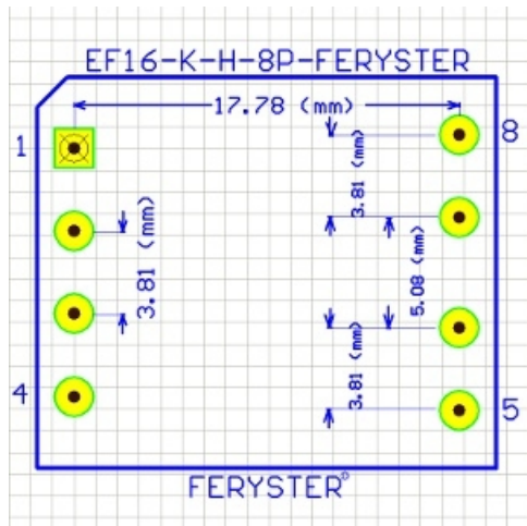
Footprint - Top view
