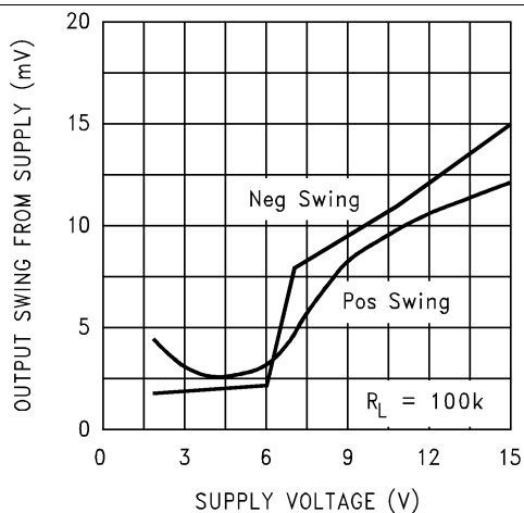
Figure 29. Output Voltage Swing vs Supply Voltage
