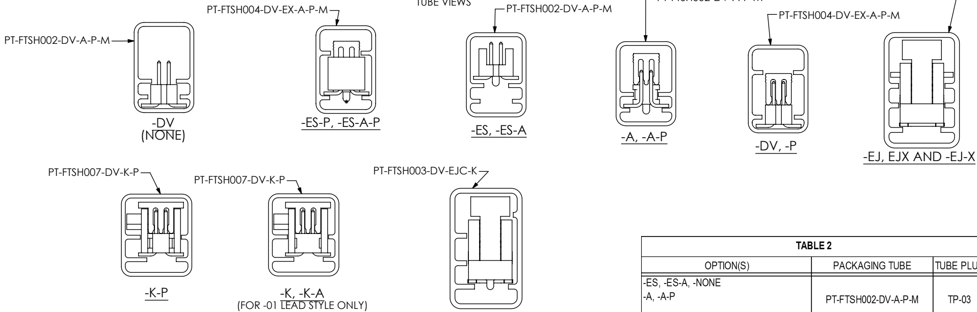
FIG 13 TUBE VIEWS
