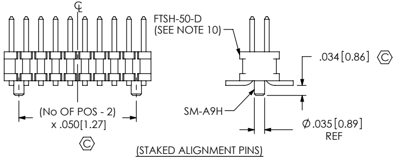
FIG 3 -A OPTION
