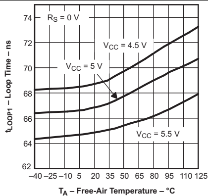
Figure 1. Recessive-to-Dominant Loop Delay vs Free-Air Temperature
