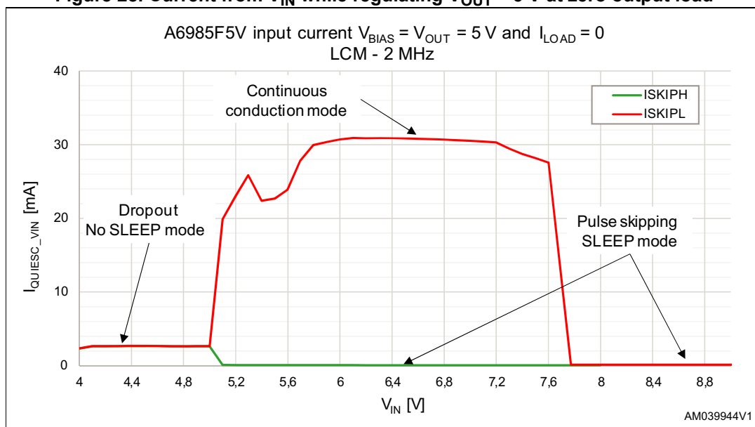
Figure 28. Current from V_{IN} while regulating V_{OUT} = 5\text{ V} at zero output load
