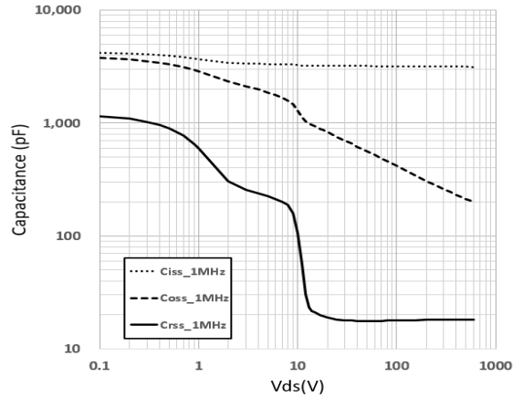
Figure 13. Capacitance Charge
