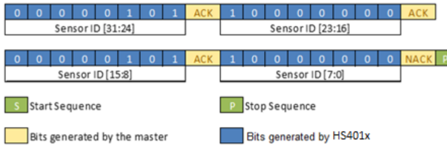
Figure 22. Read Sensor ID Command Sequence
