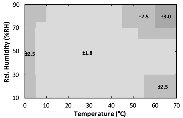
Figure 4. HS4012 RH Accuracy over Temperature
