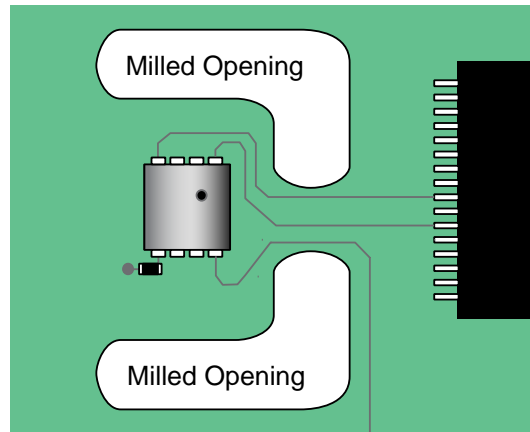
Figure 25. Milled PCB Openings for Thermal Isolation
