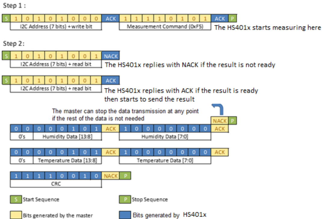
Figure 15. Typical No-Hold Measurement Sequence for a Humidity and Temperature Command
