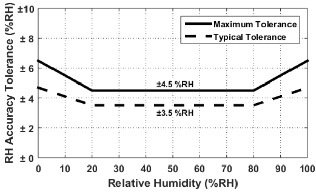
Figure 7. HS4014 RH Accuracy Tolerance at 25°C
