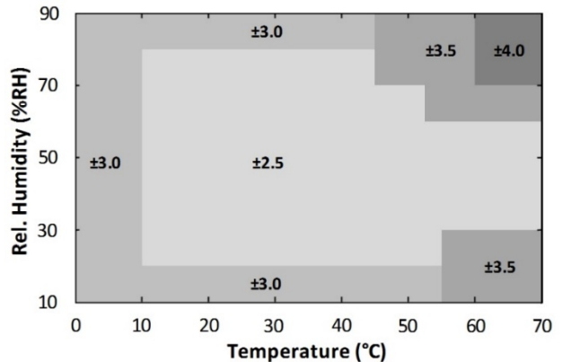
Figure 6. HS4013 RH Accuracy over Temperature
