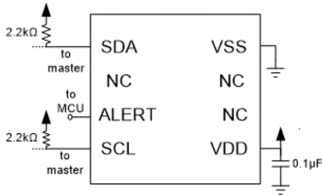
Figure 23. HS401x Application Circuit (Top View)
