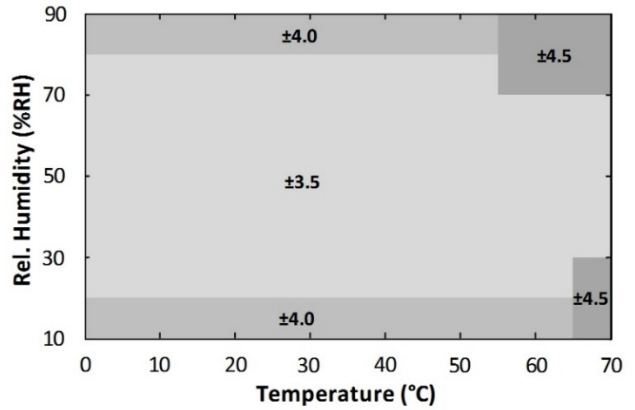
Figure 8. HS4014 RH Accuracy over Temperature
