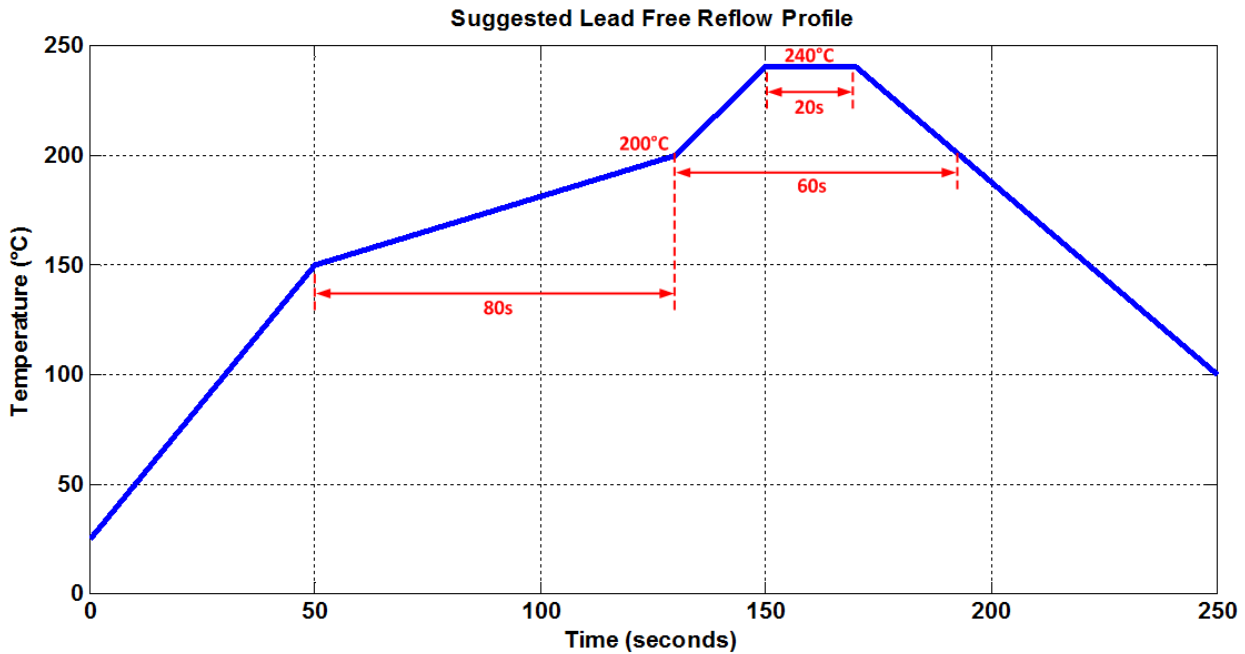
Figure 24. Recommended Soldering Profile
