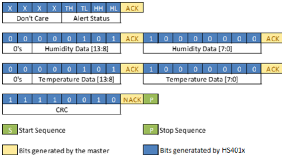
Figure 19. Data Returned from HS401x when the Alert Feature is Enabled in Periodic Measurement Mode
