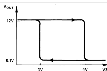
Figure 38. V_{OUT} vs V3
