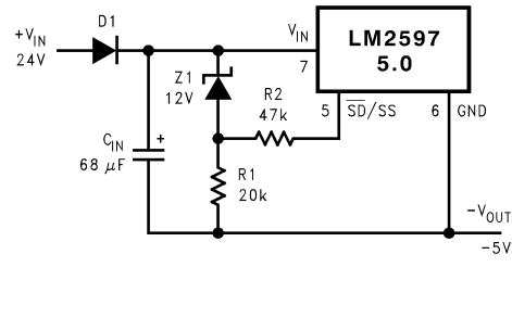
Figure 28. Undervoltage Lockout With Hysteresis for an Inverting Regulator
