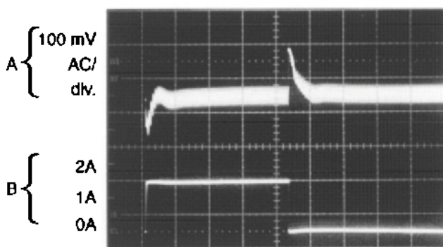
Figure 15. Horizontal Time Base: 2 \mu\text{s}/\text{div}
