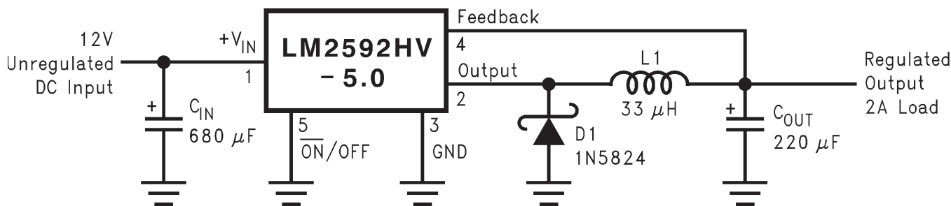
Figure 27. Typical Application
