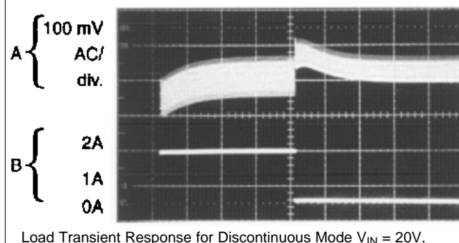
Figure 16. Horizontal Time Base: 2 \mu\text{s}/\text{div}
