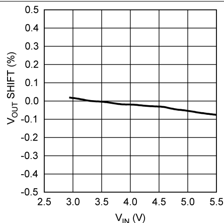
Figure 10. Line Regulation
