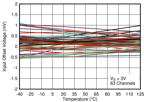
Figure 7-12. Input Offset Voltage vs. Temperature at 3V
