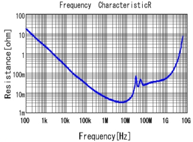
■ LLL31MR71E474MA01 R DCOV, 25degC
