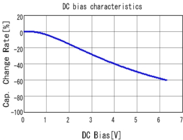
■ LLL153C80J224ME14 C-DC bias capchange, 25.0degC, AC0.
