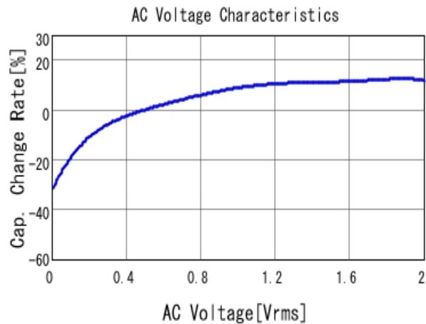
■ LLL153C80J224ME14 C-AC Voltage capchange, DCOV, 25.0d
