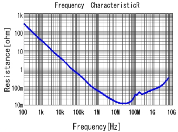
■ LLL153C80J224ME14 R DCOV, 25degC
