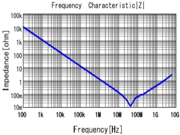
■ LLL153C80J224ME14 |Z| DCOV, 25degC
