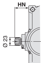
End lock mechanism (Manual release lock type)
