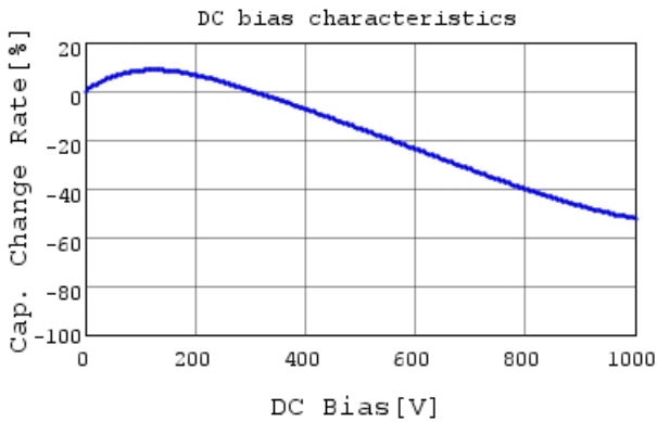
DE1E3RA222MN4AP01F C-DC bias capchange, 20.0
