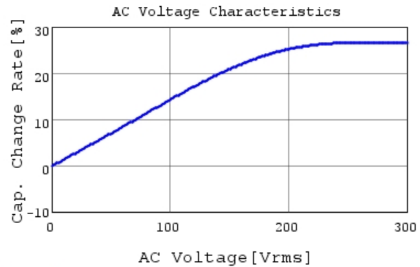
DE1E3RA222MN4AP01F C-AC Voltage capchange, I
