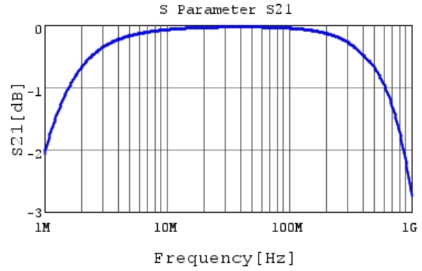
DE1E3RA222MN4AP01F S21 DCOV, 20degC
