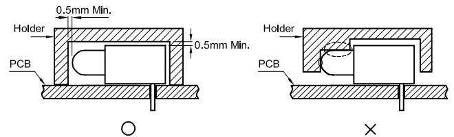
" ○ " Correct mounting method " x " Incorrect mounting method
