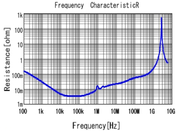
■ KCM55WR7YA476MH01 R DCOV, 25degC
