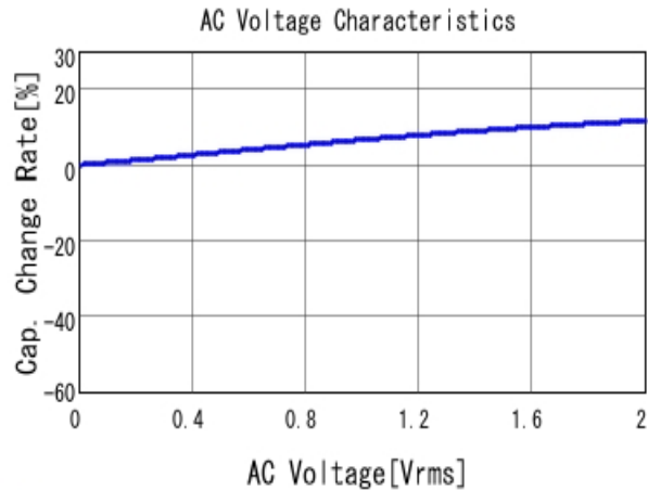
■ KCM55WR7YA476MH01 C-AC Voltage capchange, DCOV, 25.0d
