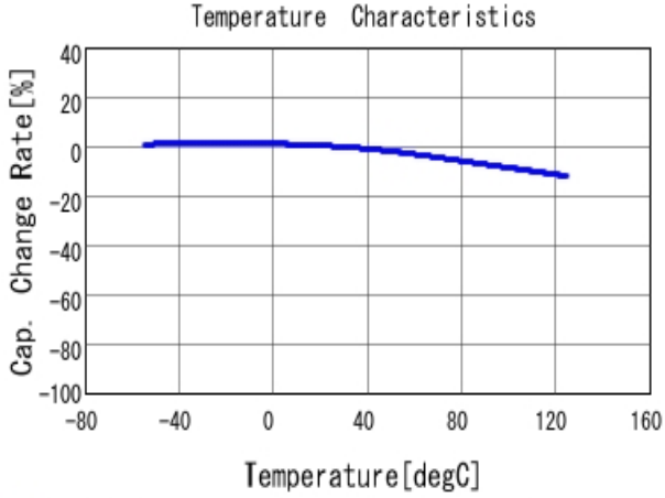
■ KCM55WR7YA476MH01 C-Temp. capchange, DCOV, ACO, 5Vrms
