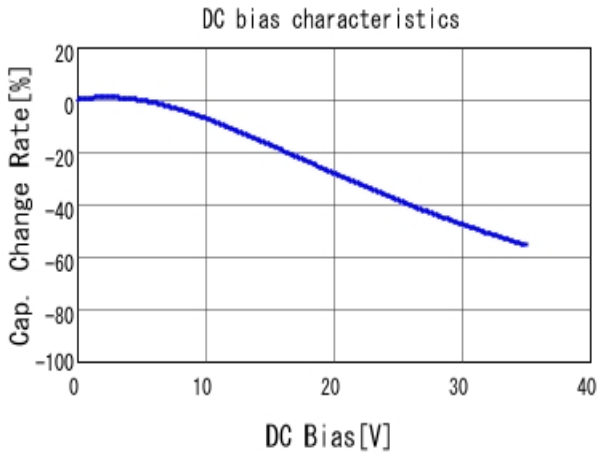
■ KCM55WR7YA476MH01 C-DC bias capchange, 25.0degC, AC0.
