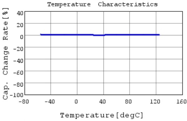
KCM55WR71H336MH01 C-Temp. capchange, DCOV, 1
