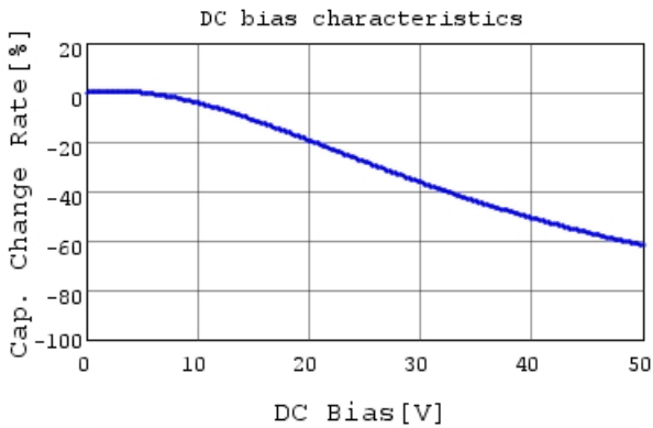
KCM55WR71H336MH01 C-DC bias capchange, 25.0c
