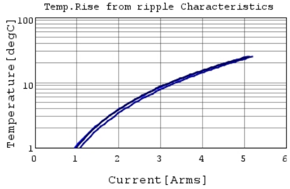
KCM55WR71H336MH01 Temp.rise 50kHz
