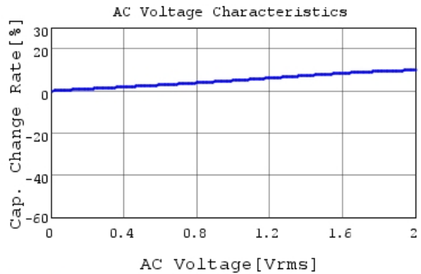
KCM55WR71H336MH01 C-AC Voltage capchange, Dc
