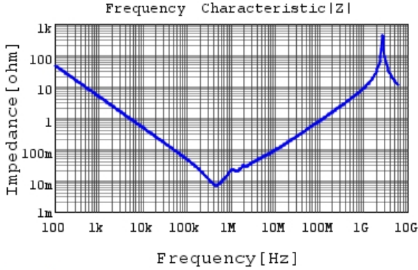
KCM55WR71H336MH01 |Z| DCOV, 25degC
