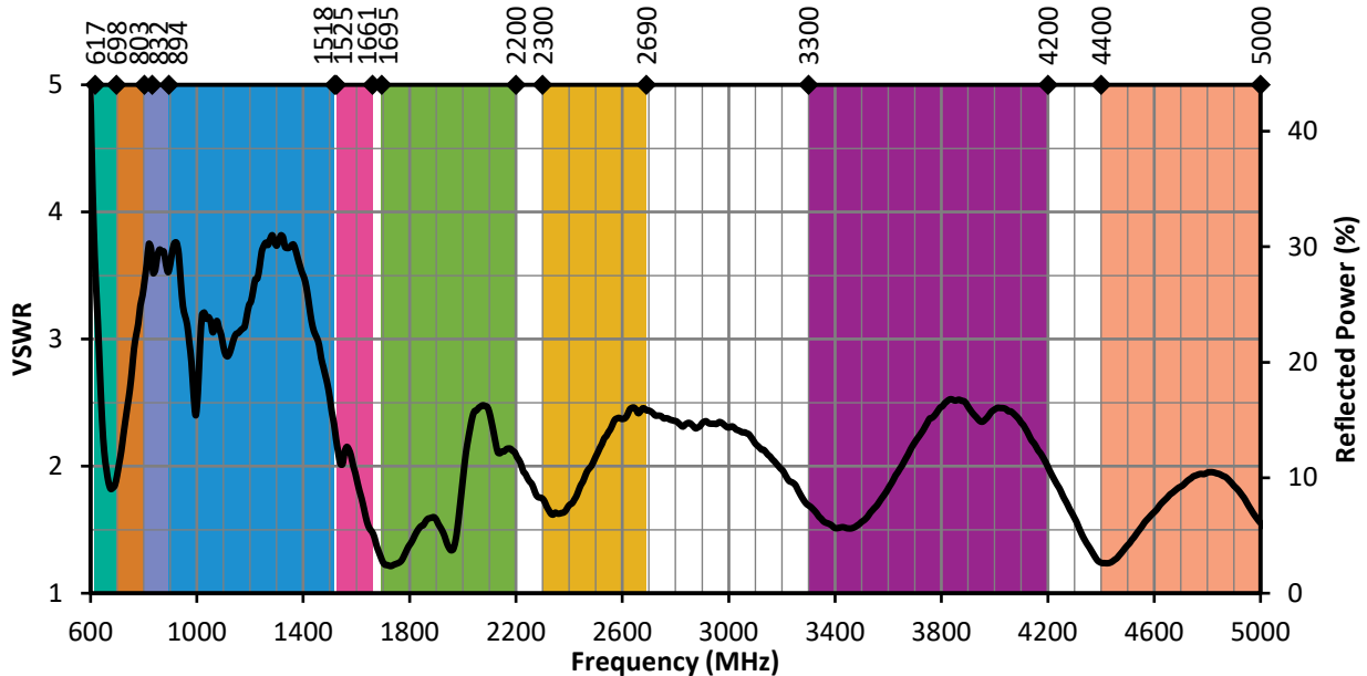
Figure 11. ANT-5GWWS3-SMA VSWR, Edge-Bent
