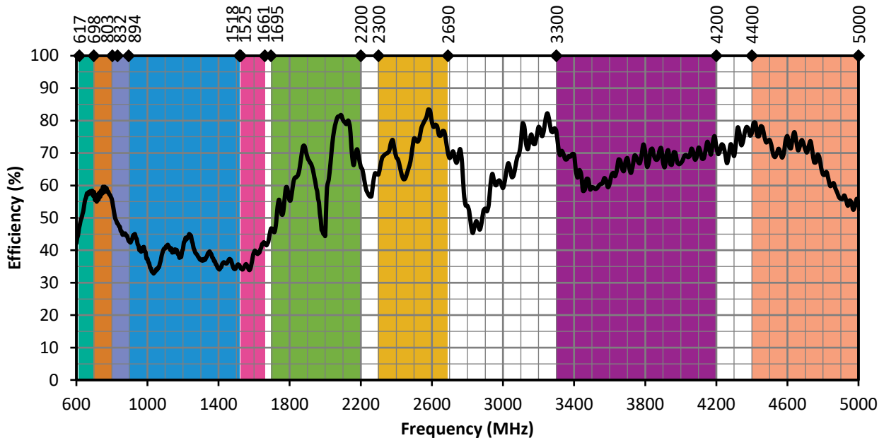
Figure 8. ANT-5GWWS3-SMA Antenna Efficiency, Straight
