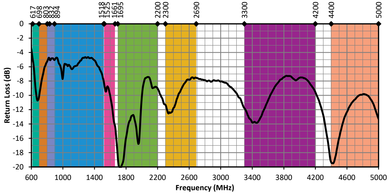
Figure 12. ANT-5GWWS3-SMA Return Loss, Edge-Bent
