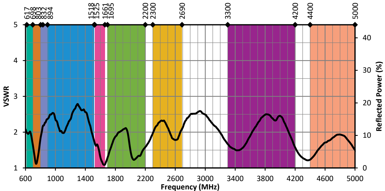
Figure 4. ANT-5GWWS3-SMA VSWR, Straight
