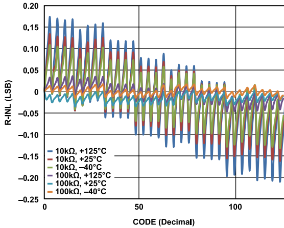
Figure 9. R-INL vs. Code (AD5121)
