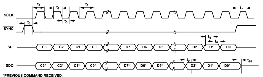
Figure 4. SPI Serial Interface Timing Diagram, CPOL = 0, CPHA = 1
