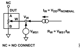
Figure 37. Wiper Resistance
