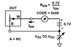
Figure 39. Incremental on Resistance
