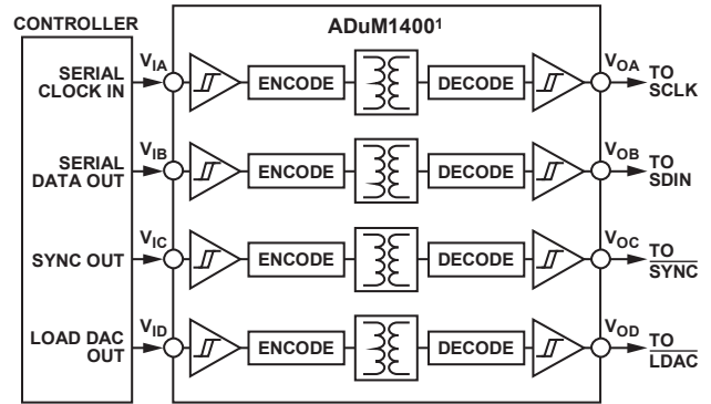
Figure 54. Isolated Interface
