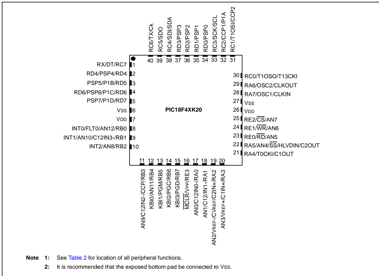
FIGURE 4: 40-PIN UQFN
