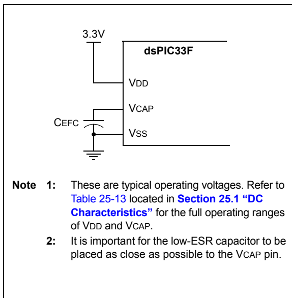
FIGURE 22-1: CONNECTIONS FOR THE ON-CHIP VOLTAGE REGULATOR (1)
