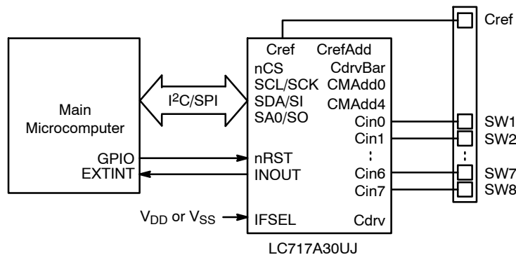
Figure 1. Application Schematic 1
