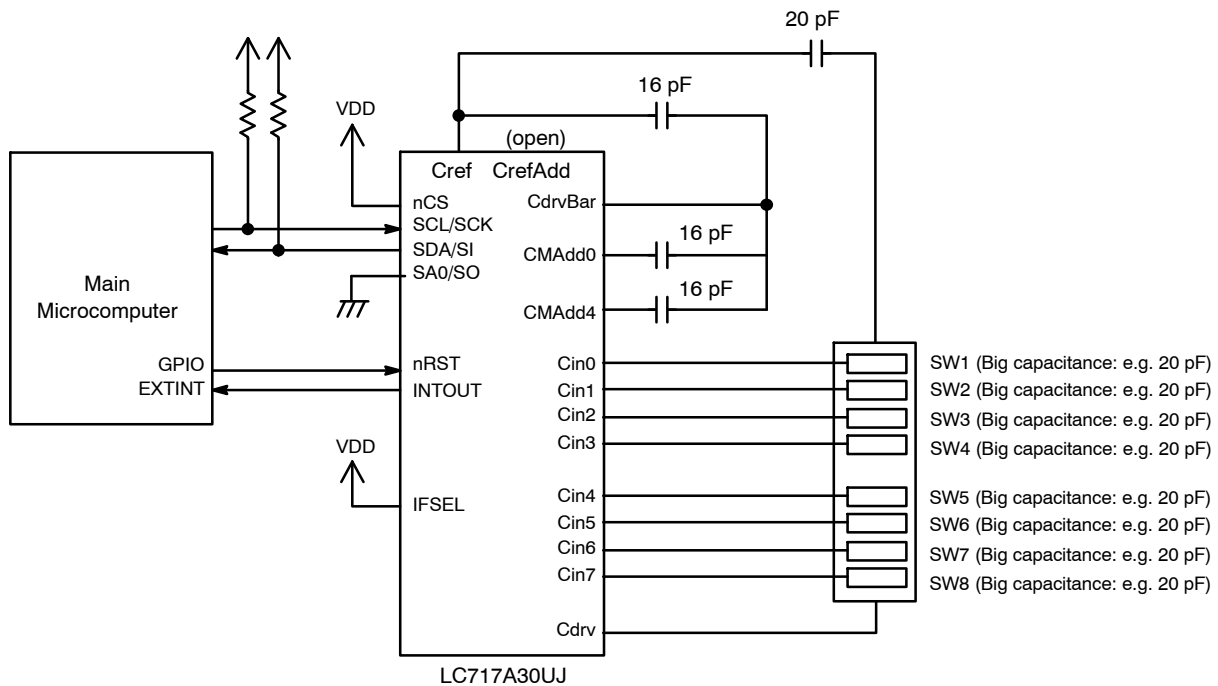
Figure 3. Application Schematic 3
