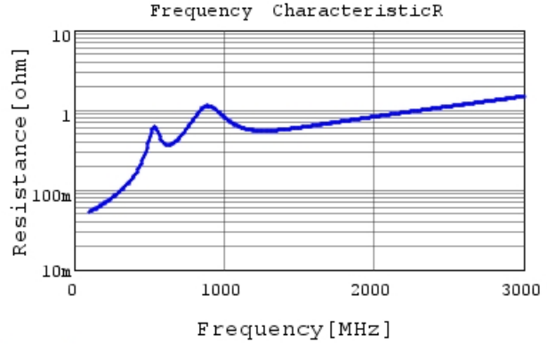
GRM31A7U2J821JW31 R DC0V, 25degC
