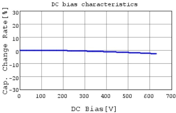
GRM31A7U2J821JW31 C-DC bias capchange, 25.0c
