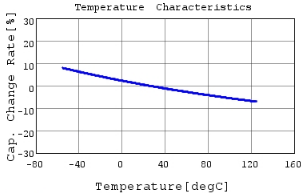
GRM31A7U2J821JW31 C-Temp. capchange, DC0V, 1
