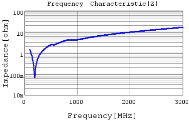
GRM31A7U2J821JW31 |Z| DC0V, 25degC
